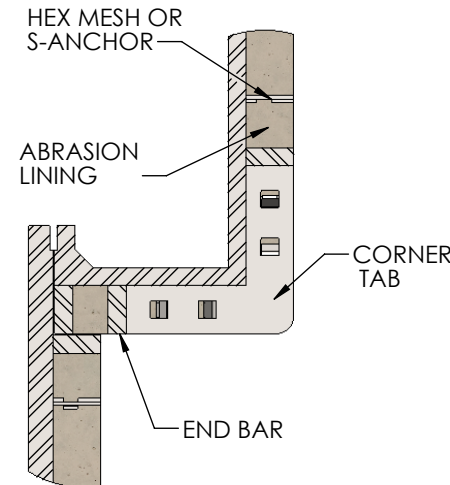
MANWAY AND NOZZLE CORNER TABS
